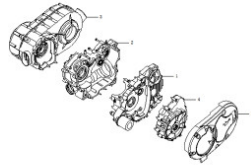
CVT Housing MICF0180-013000
